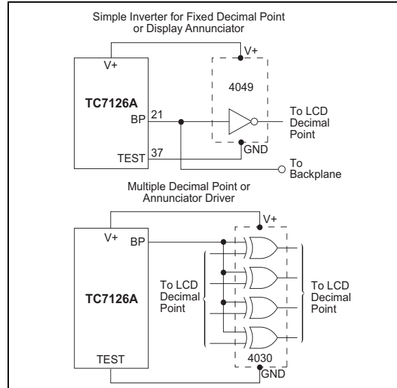
FIGURE 8-1: Decimal Point and Annunciator Drives
